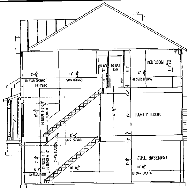
B BUILDING SECTION THROUGH STAIRS
