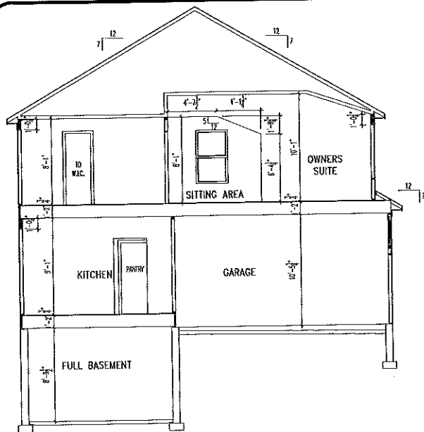
A BUILDING SECTION THROUGH GARAGE
