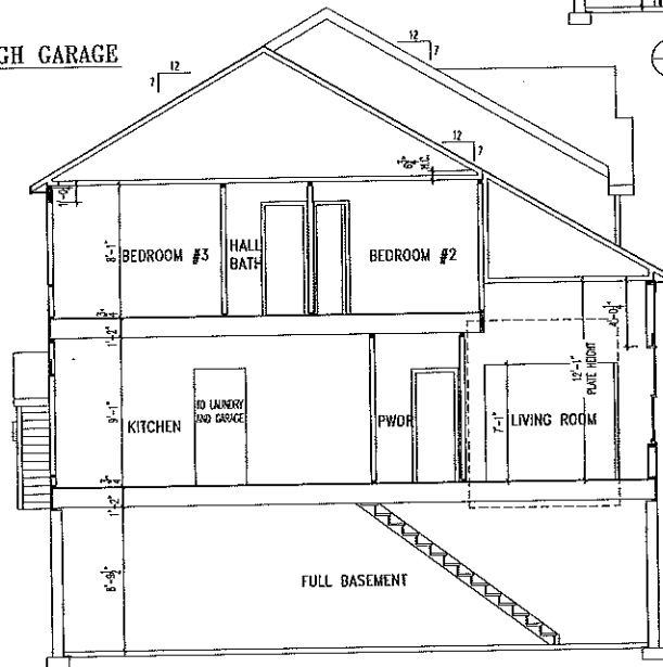
C BUILDING SECTION
